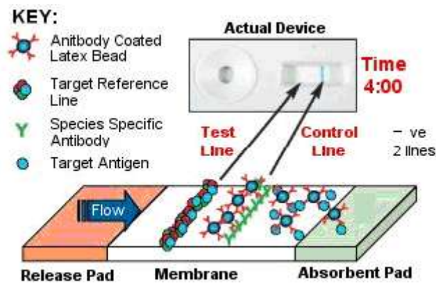
Figure 1. The Competitive lateral flow assay format
